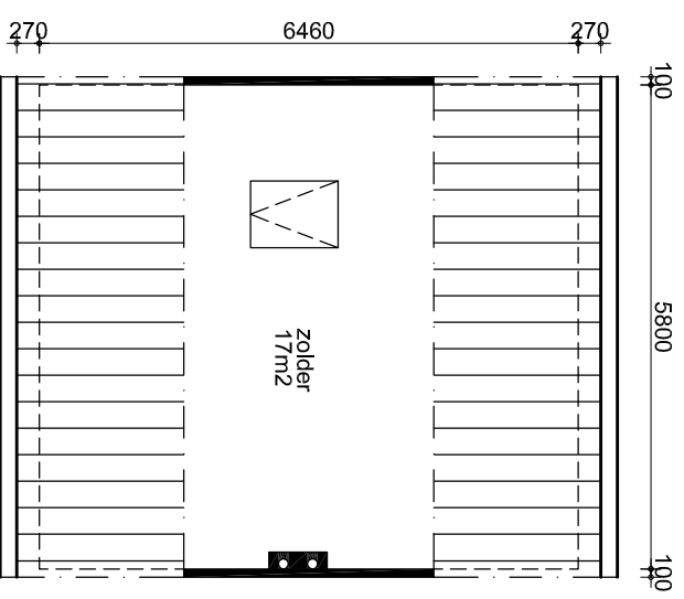
Zolder
