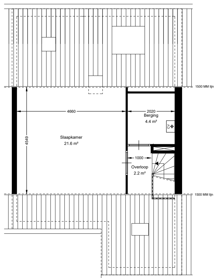
Zolder
