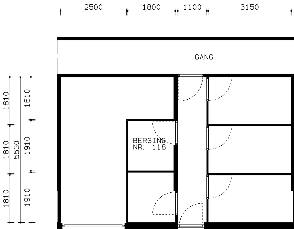
BERGING/GARAGE
